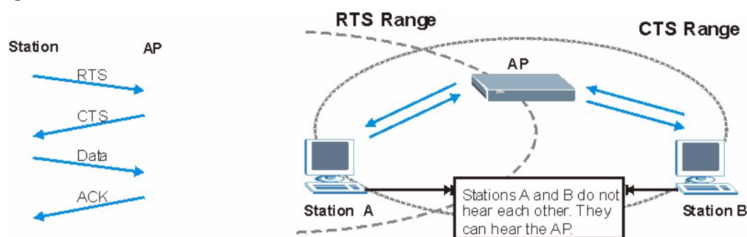
Figure 26 RTS/CTS
