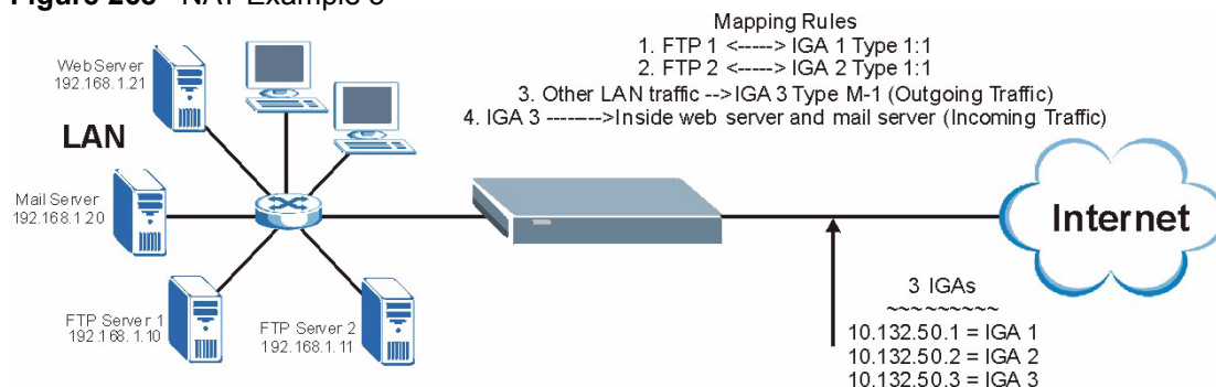
Figure 268 NAT Example 3
