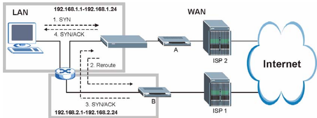
Figure 32 IP Alias
