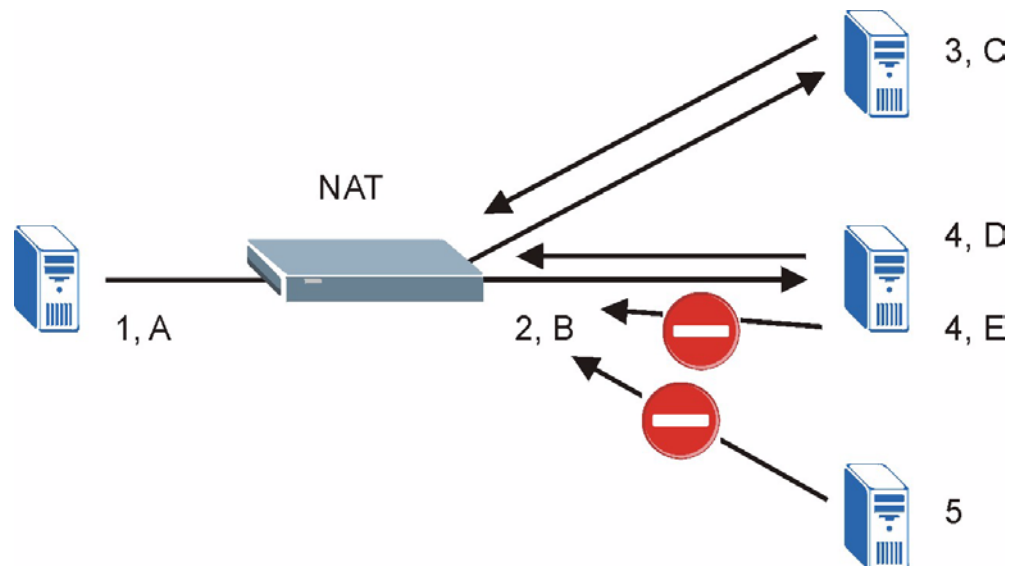
Figure 137 Port Restricted Cone NAT Example
