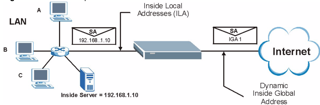
Figure 266 NAT Example 2
