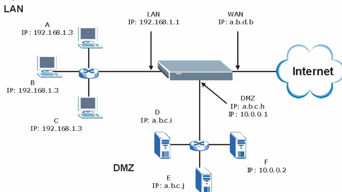
Figure 55 DMZ Private and Public Address Example
