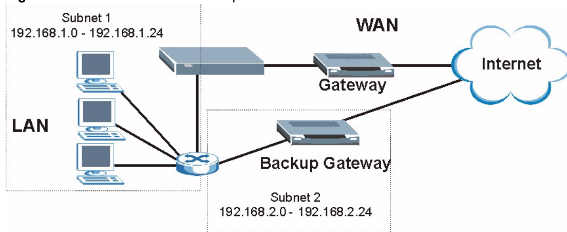
Figure 48 Traffic Redirect LAN Setup
