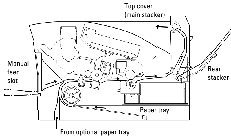
Figure 1-4 Paper paths
