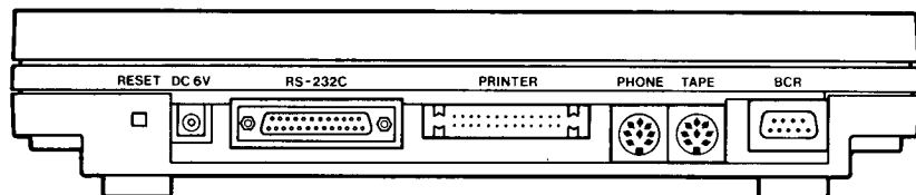
Fig. 1-9 Rear Panel Connections
