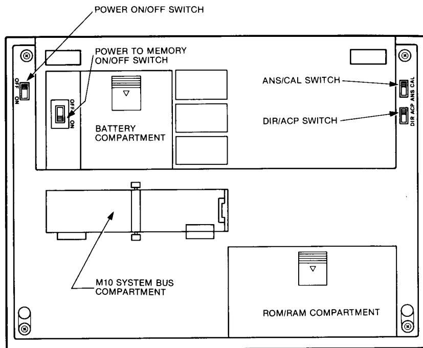
Fig. 1-10 Underside Panel
