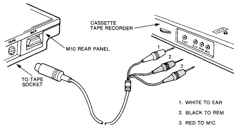
Fig. 9-1 Connecting the M10 to a Cassette Recorder
