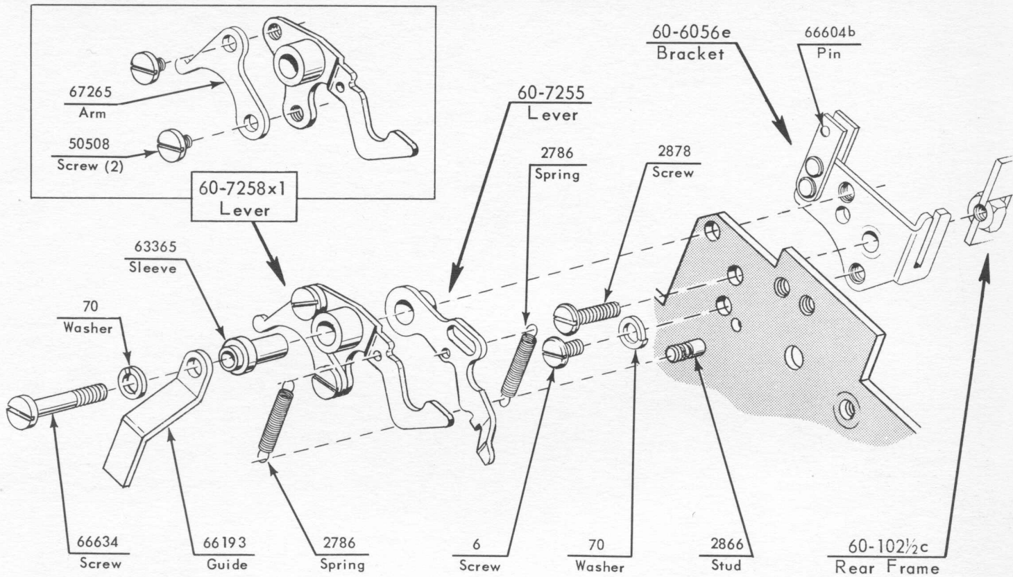
10 BANK TRIP LEVER MECHANISM
