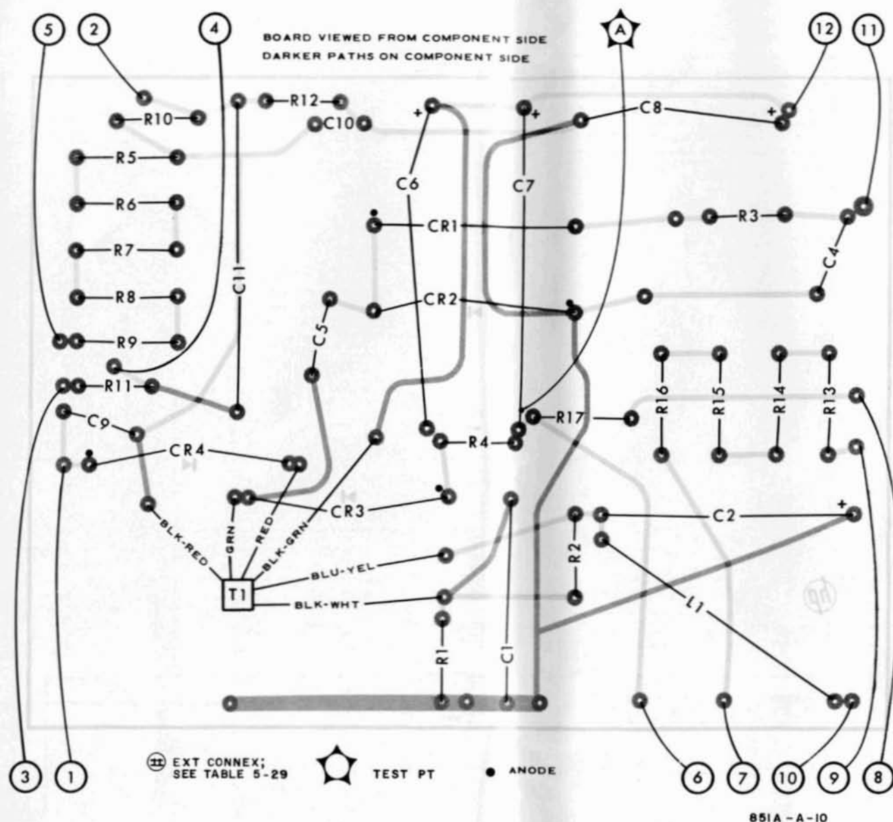
Figure 5-34. HV Power Supply A8 Board
