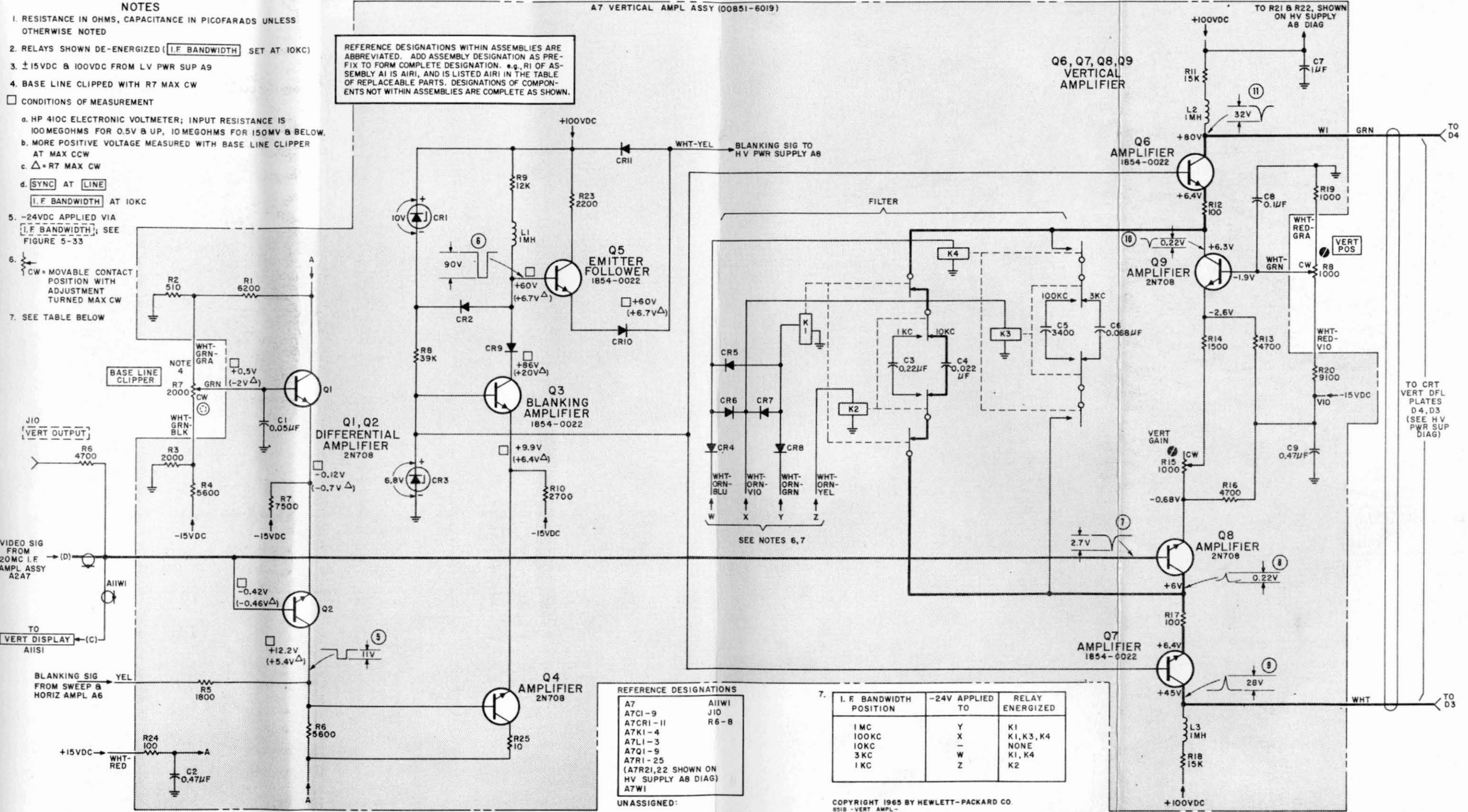
Figure 5-29. Vertical Amplifier Schematic, 851B
