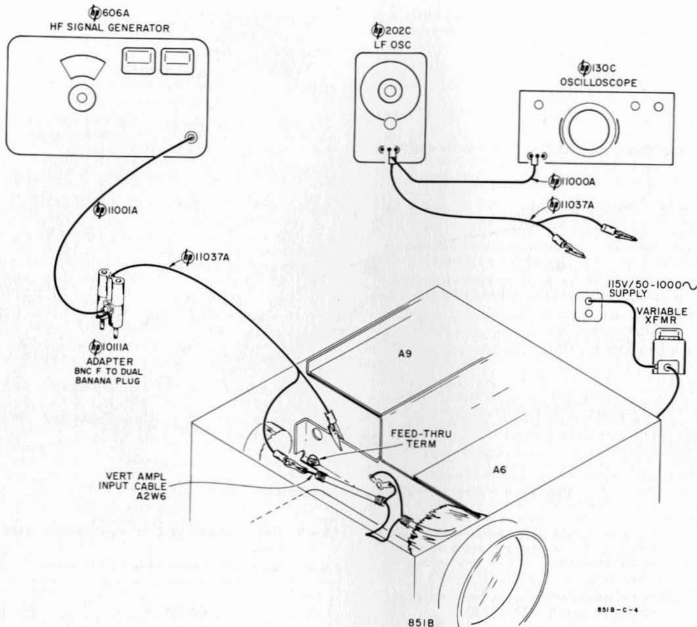
Figure 5-6. Setup for 851 Video Bandwidth Measurements
