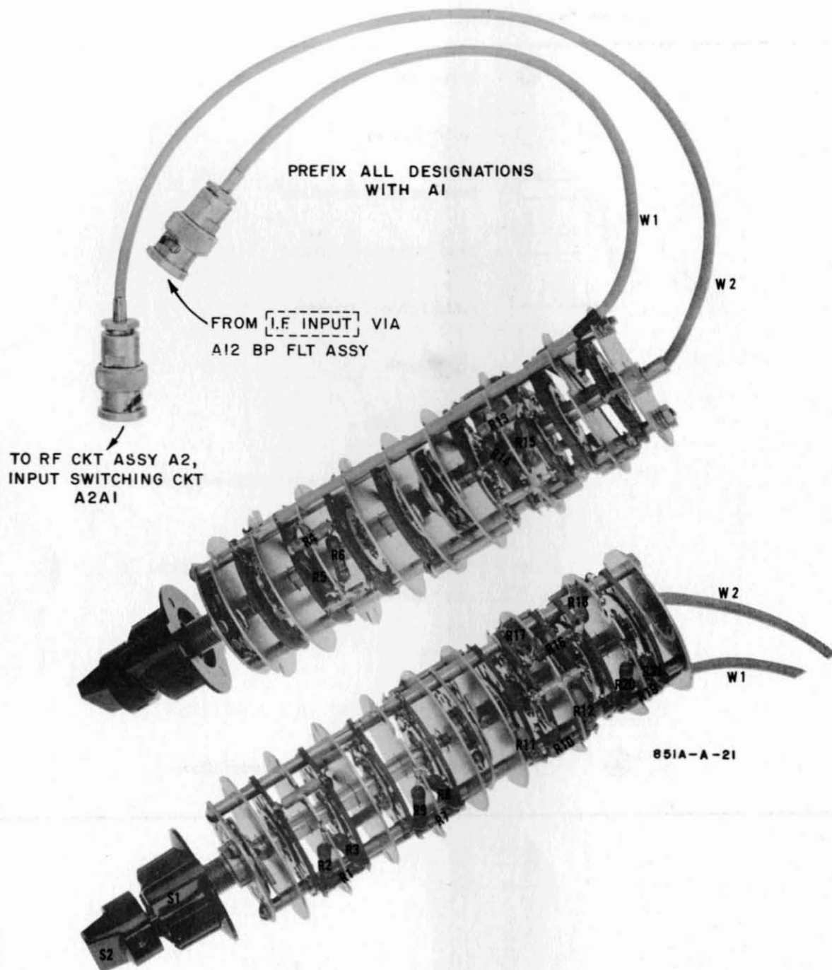
Figure 5-18. I. F. GAIN (DB) Switch Assembly A1, Component Identification
