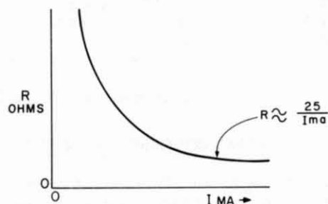
Figure 4-4. Typical Dynamic Resistance-vs-Current Curve, Hot Carrier Diodes
