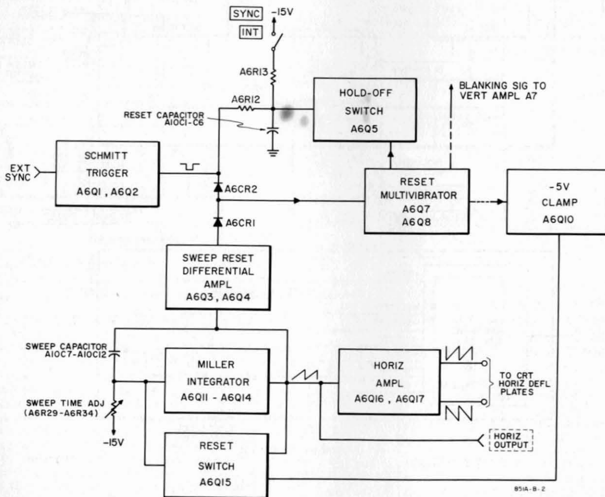
Figure 4-3. Horizontal Sweep Generator, Block Diagram
