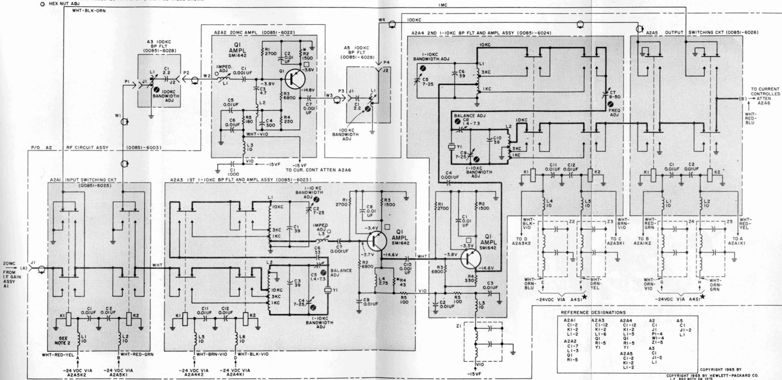
Figure 5-24. I. F. Bandwidth Switching Circuits, 851B
