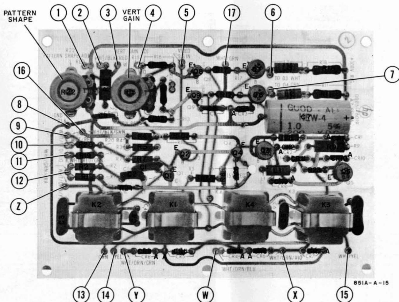
Figure 5-28. Vertical Amplifier A7 Board
