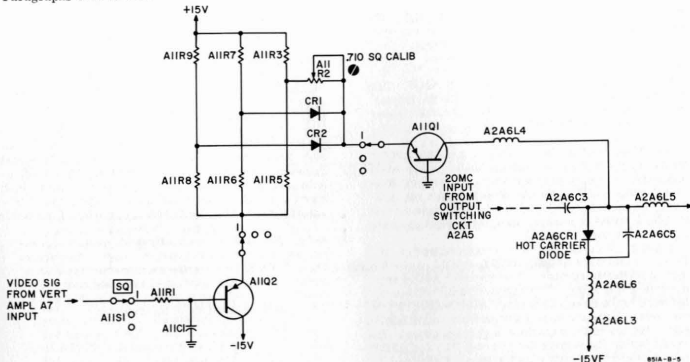
Figure 4-5. VERT DISPLAY Switch at SQ, Simplified Schematic
