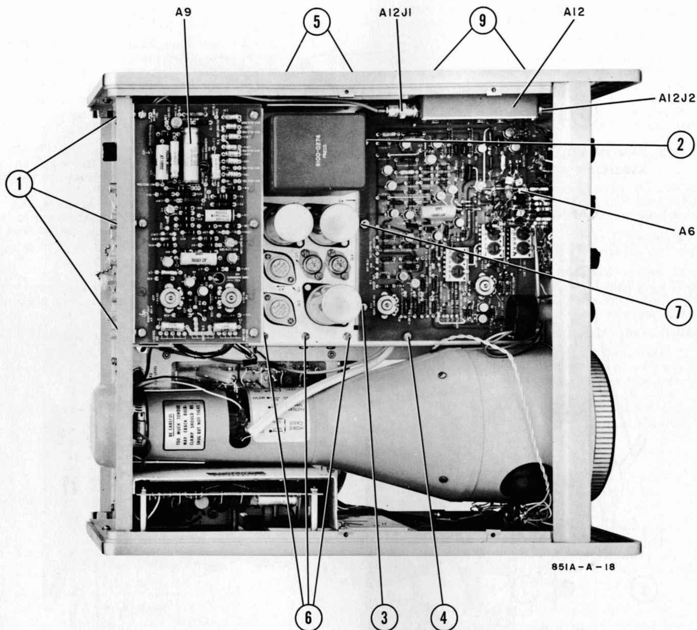
Figure 5-13. Top View of 851 Display Section
