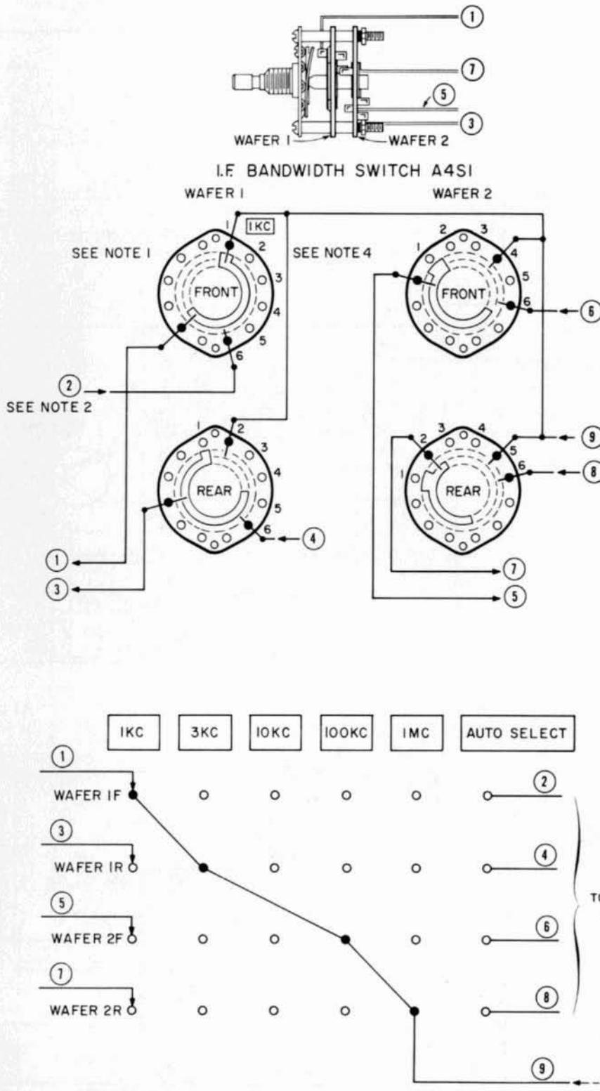
Figure 5-38. I. F. BANDWIDTH Switch A4S1
