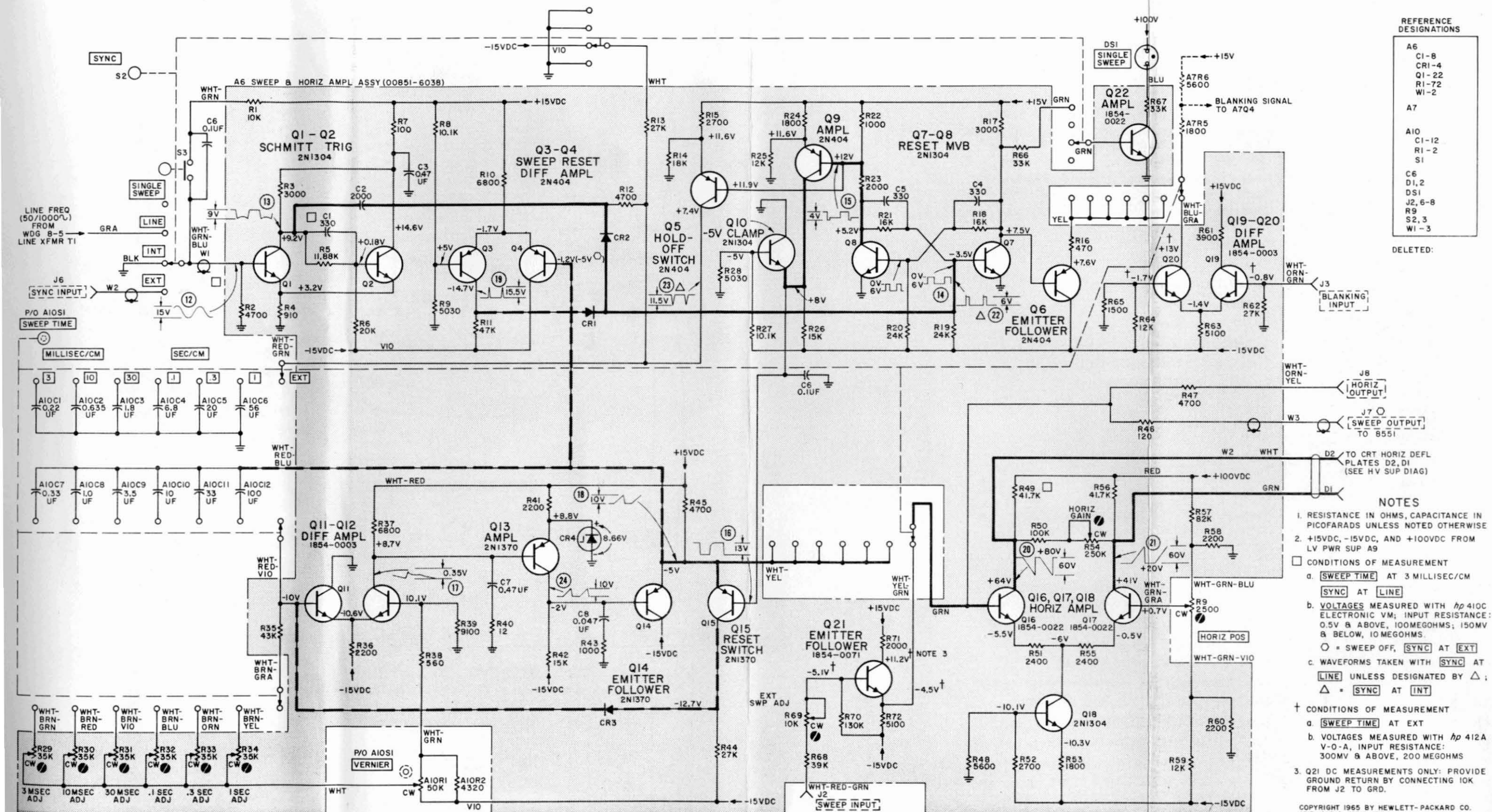
Figure 5-33. Sweep and Horizontal Amplifier Schematic, 851B
