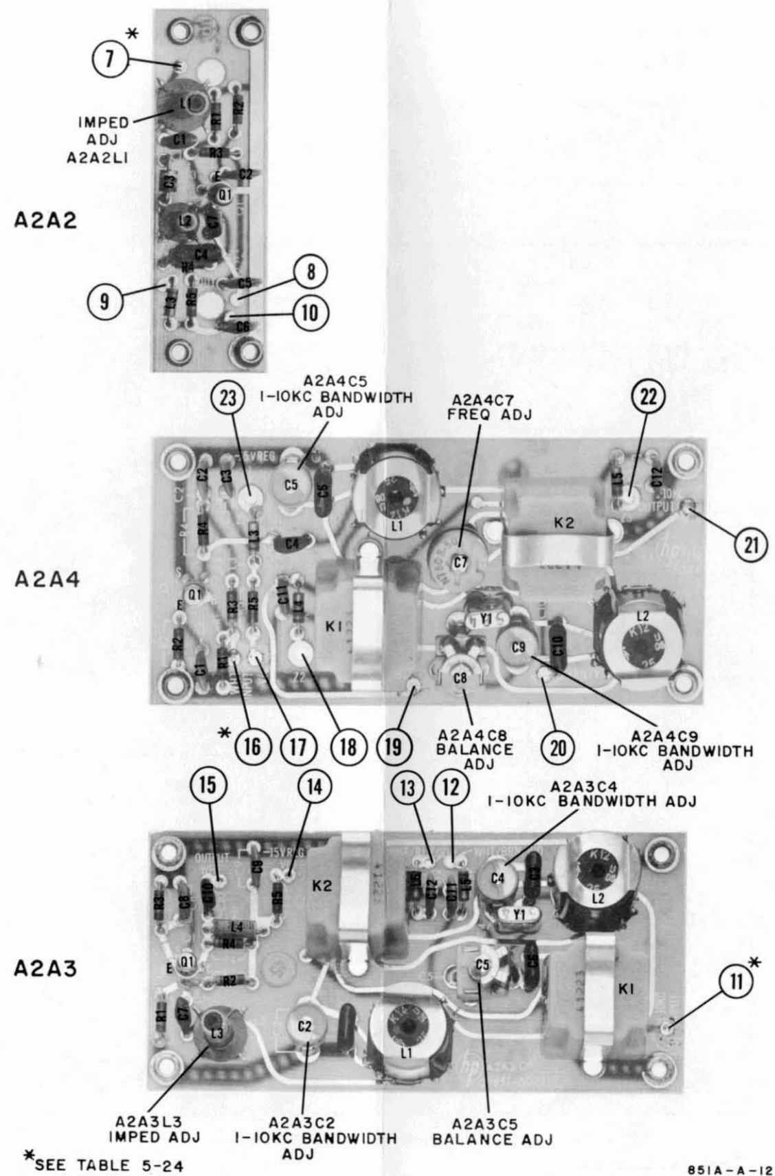
Figure 5-21. RF Circuit Assembly Boards A2A2, A2A3, A2A4
