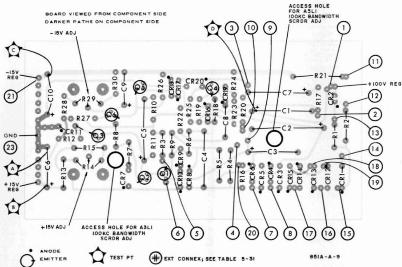
Figure 5-36. LV Power Supply A9 Board
