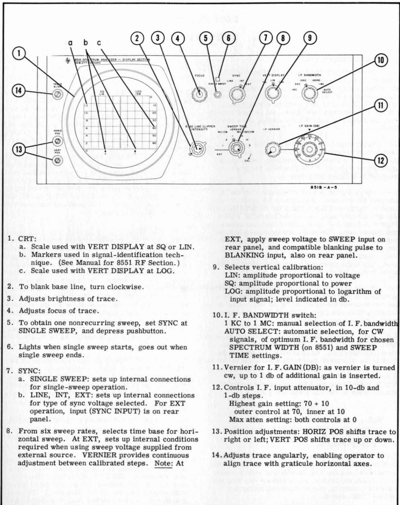
Figure 3-1. Front Panel Controls, Connectors, and Indicators, Model 851B Spectrum Analyzer Display Section
