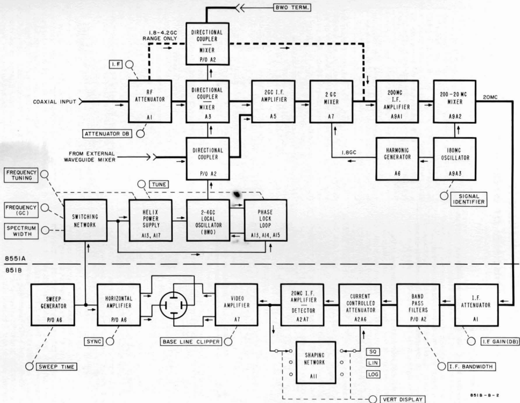
Figure 4-1. Model 851B/8551A Spectrum Analyzer, Block Diagram
