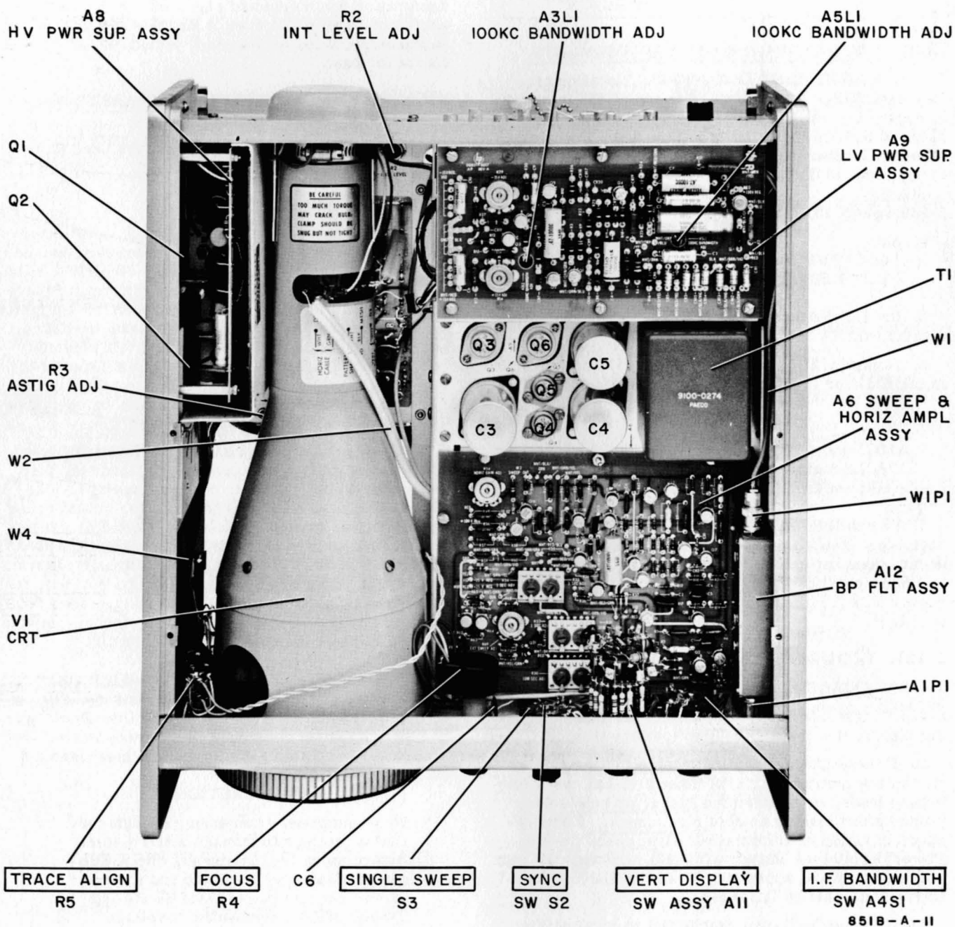
Figure 5-10. 851B Spectrum Analyzer Display Section, Top View, Top Cover Removed
