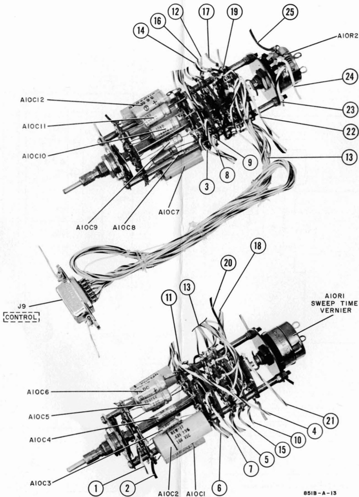
Figure 5-30. SWEEP TIME Switch A10S1, Component Identification (see Table 5-28)
