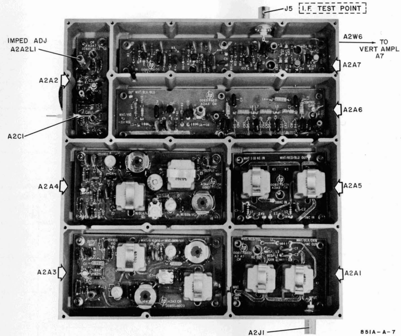
Figure 5-22. RF Circuit Assembly A2, Top Cover Removed
