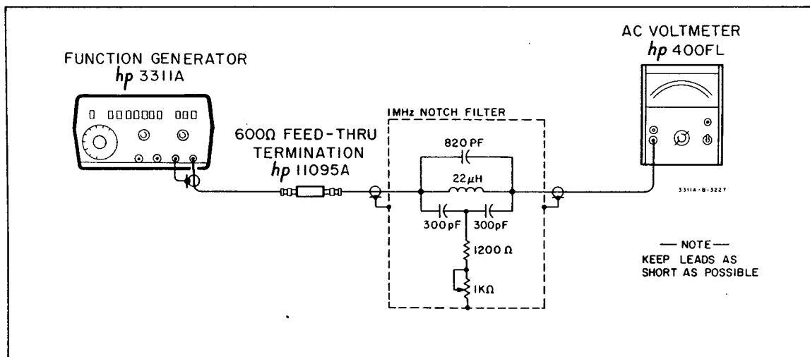
Figure 5-4. 1 MHz Distortion Test.
