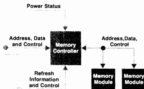
Fig. 2. Memory system is logically and physically separate from the rest of the computer. Memory runs asynchronously with the processor, synchronizing only to refresh.
