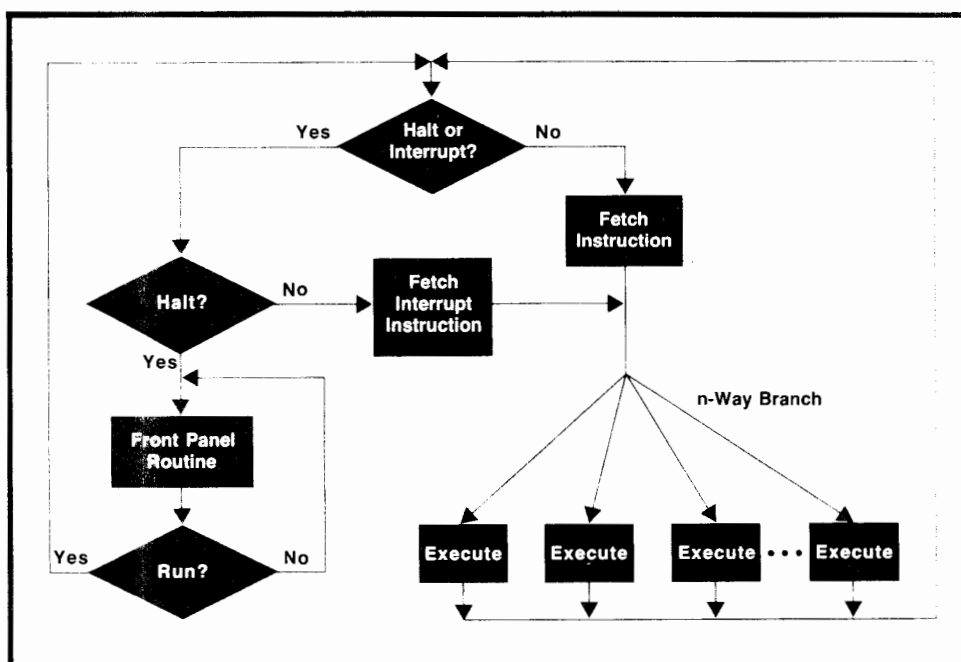
Fig. 2. 21MX microprocessor controls the front panel as well as program execution. This diagram shows the flow of control through the various machine phases.
