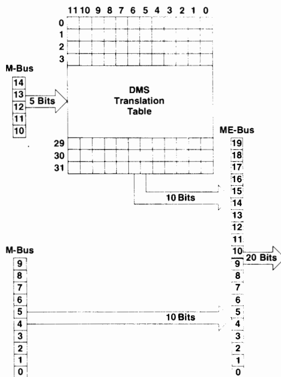
Fig. 2. DMS maps 32-page logical address space into a 1024-page physical address space. Translation tables are loaded by the operating system.
