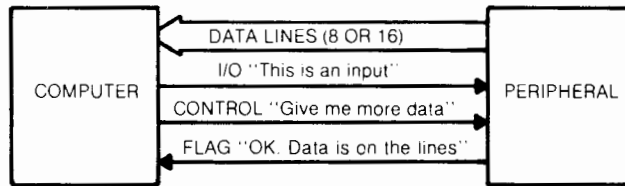
Figure I-9. Data Input Handshake
