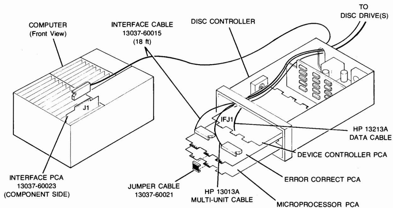
TYPICAL HP 2100A/S INSTALLATION
