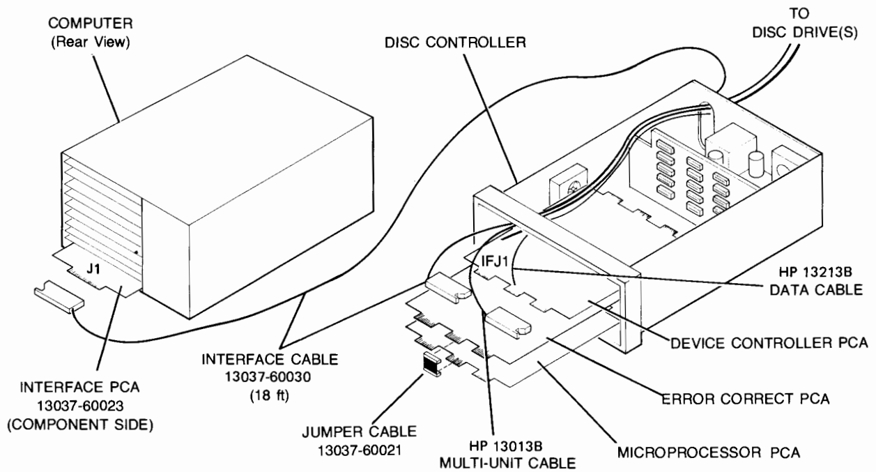
TYPICAL E-, F-, AND M-SERIES INSTALLATION
