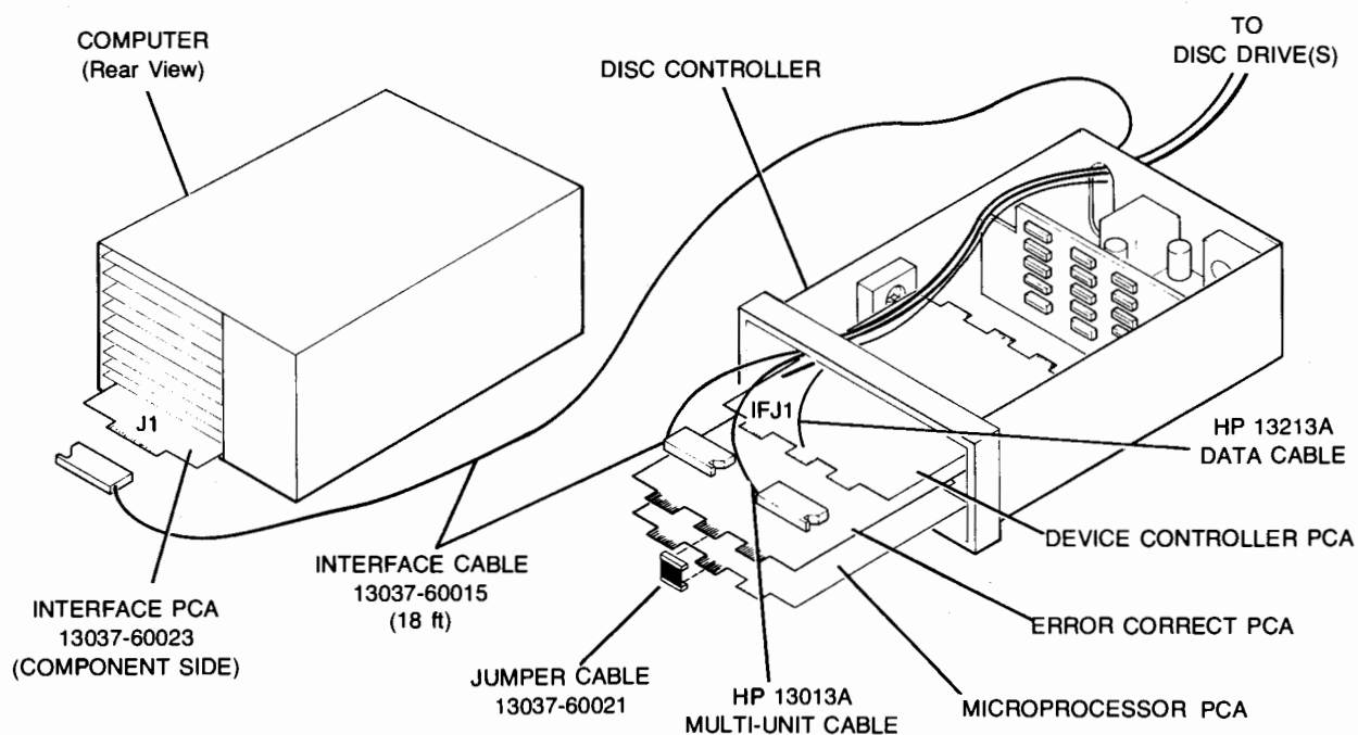
TYPICAL E- AND M-SERIES INSTALLATION
