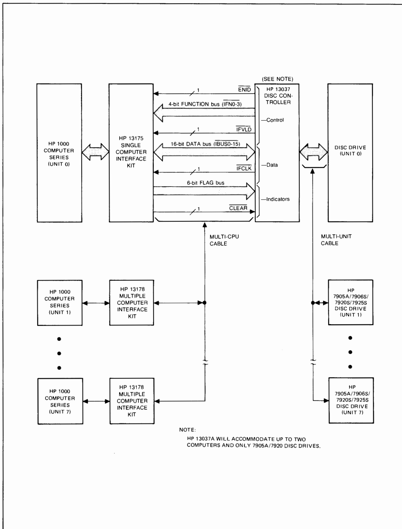
Figure 3-1. Interface PCA to Disc Controller, Block Diagram
