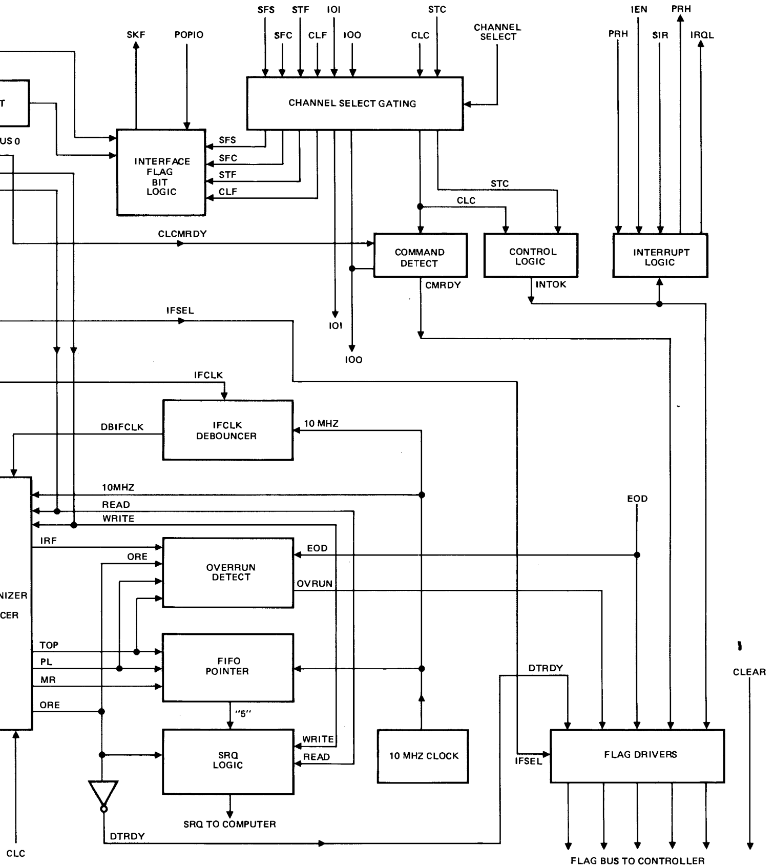
Figure 3-2. Interface PCA Functional Block Diagram
