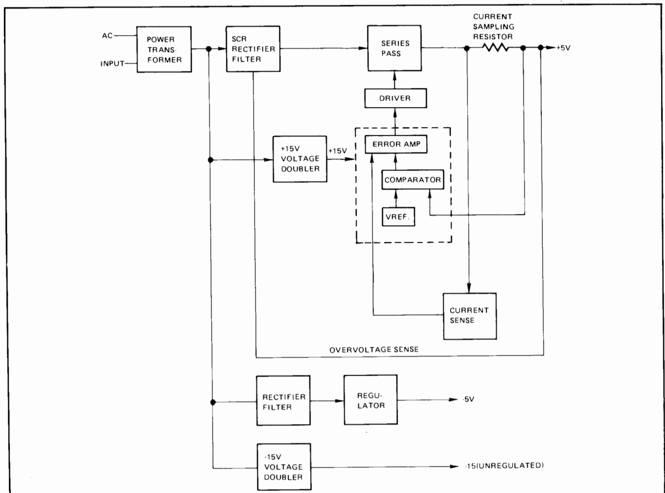
Figure A-4. Power Supply Functional Block Diagram
