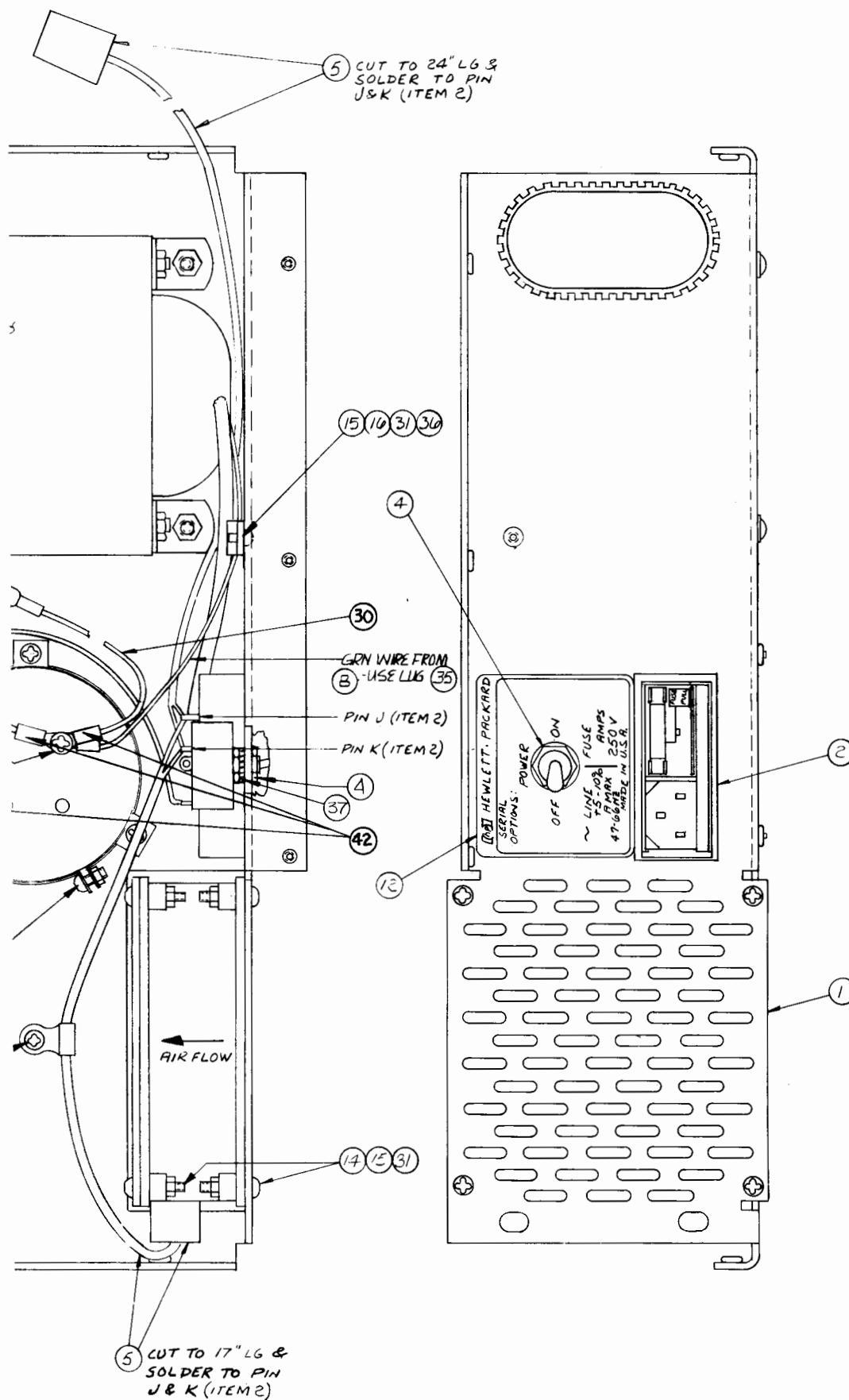
Figure A-8. Rear Deck Assembly
