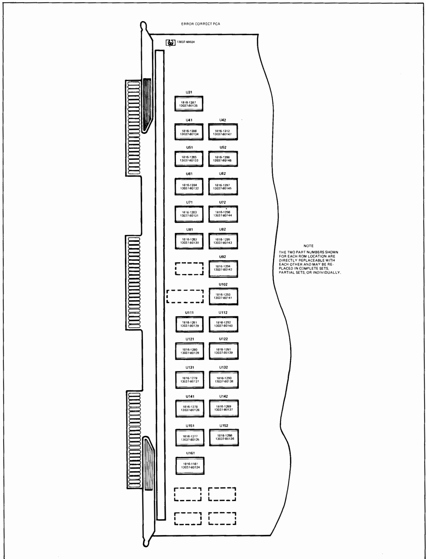
Figure 5-3. Error Correct PCA ROM Locations
