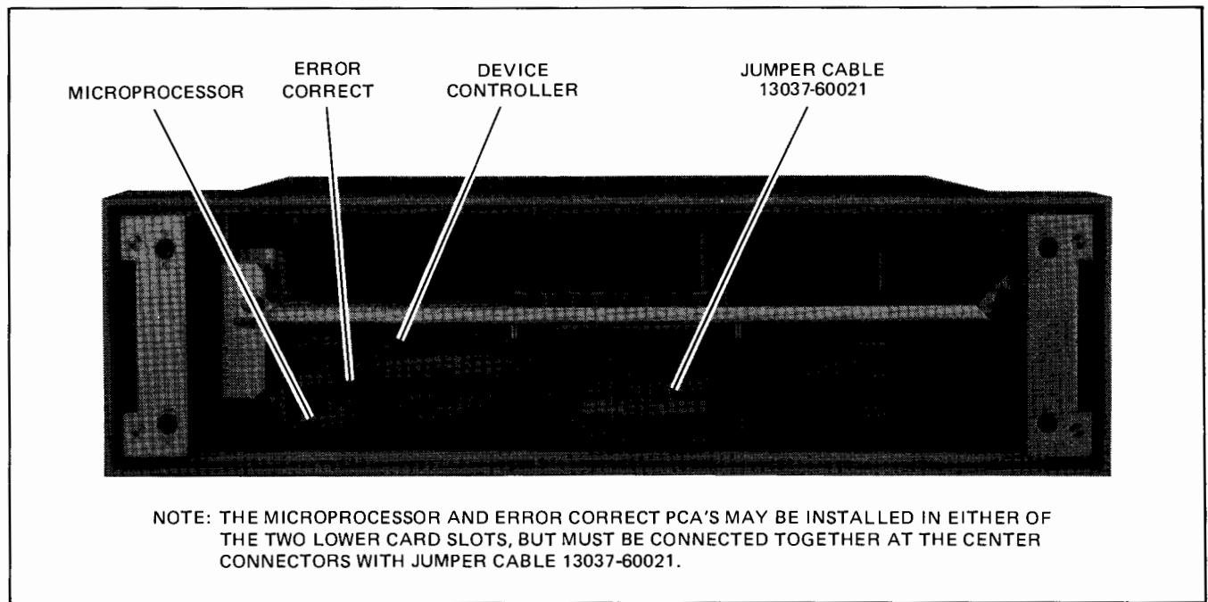
Figure 2-4. Controller PCA Configuration
