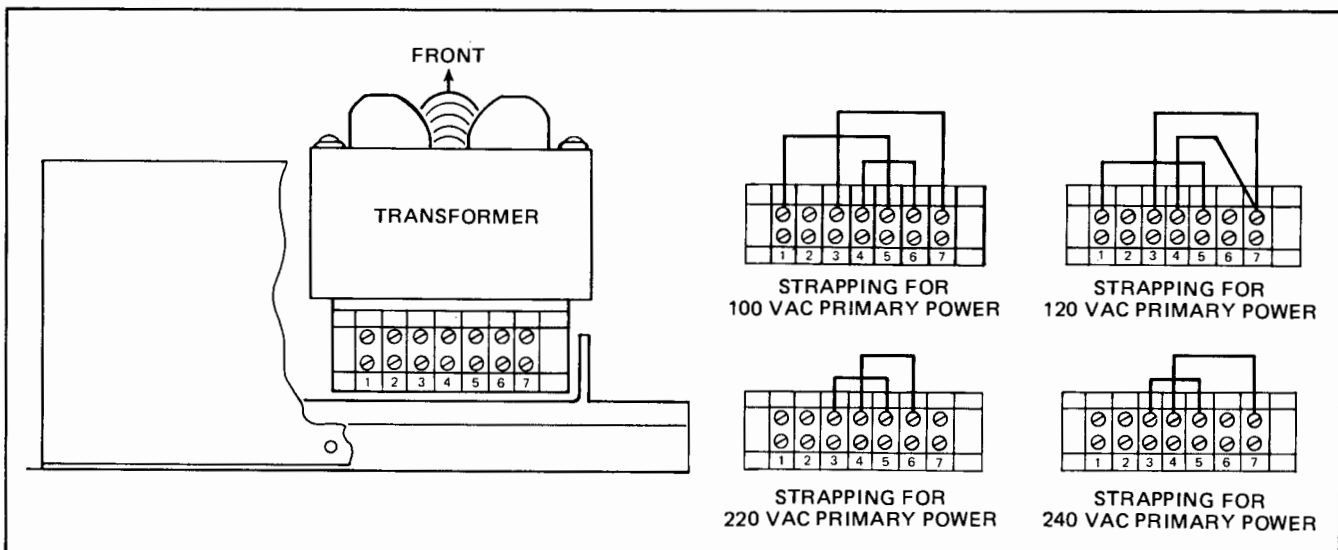
Figure 2-1. Transformer Strapping Configurations
