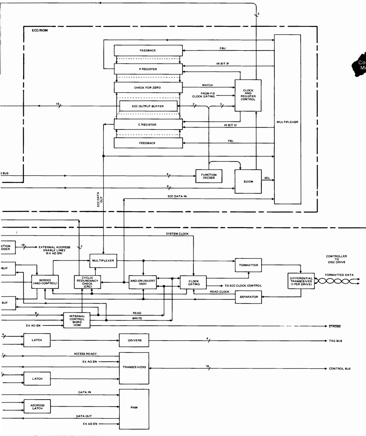
Figure 4-12. Controller Detailed Functional Block Diagram
