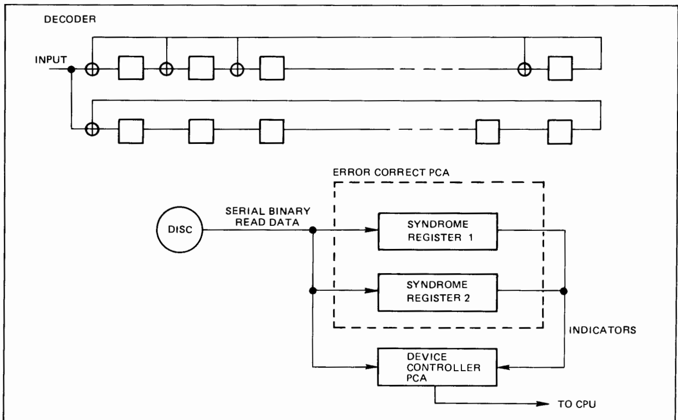
Figure 4-10. ECC Read Circuit
