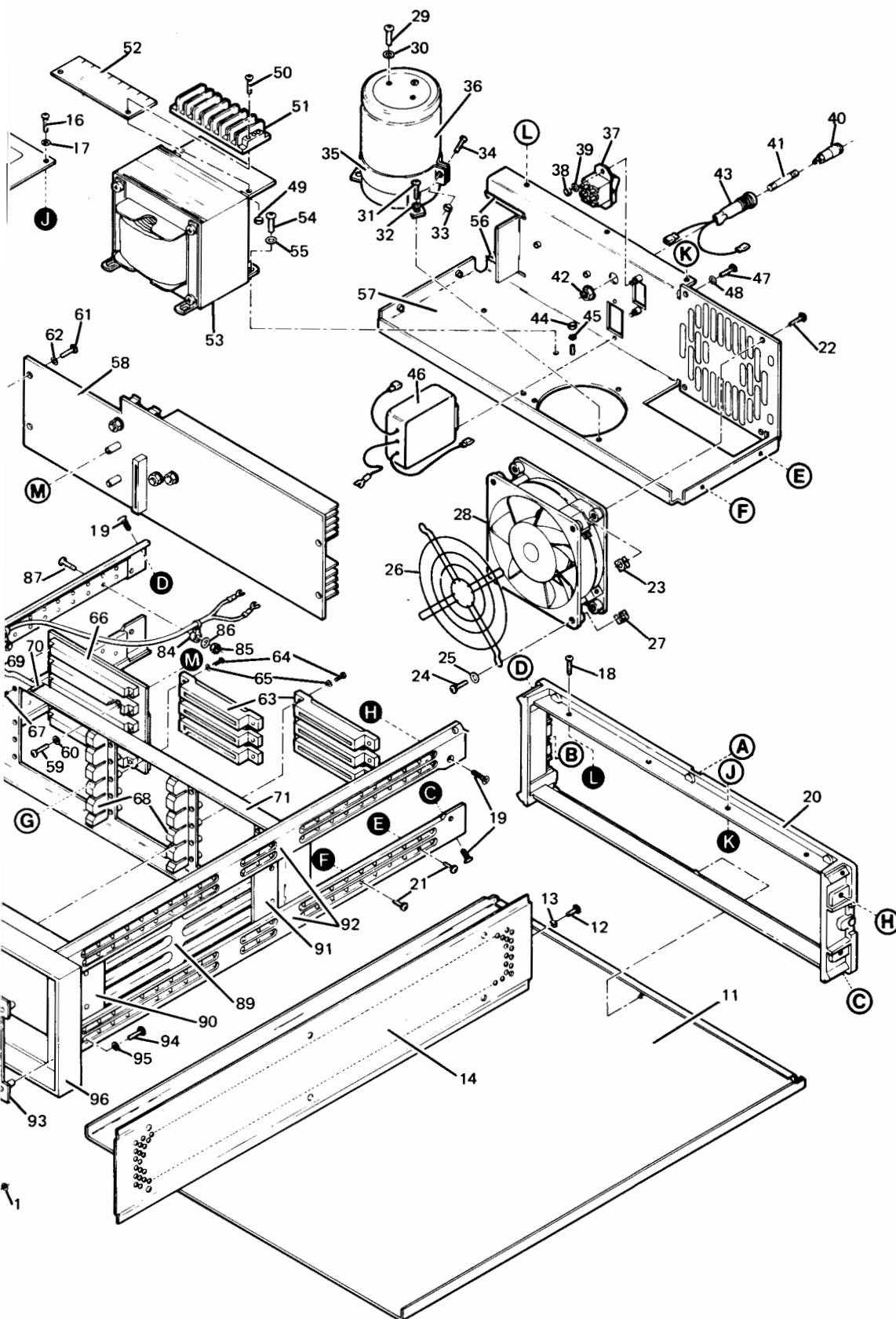
Figure 6-1. HP 13037C Controller Exploded View
