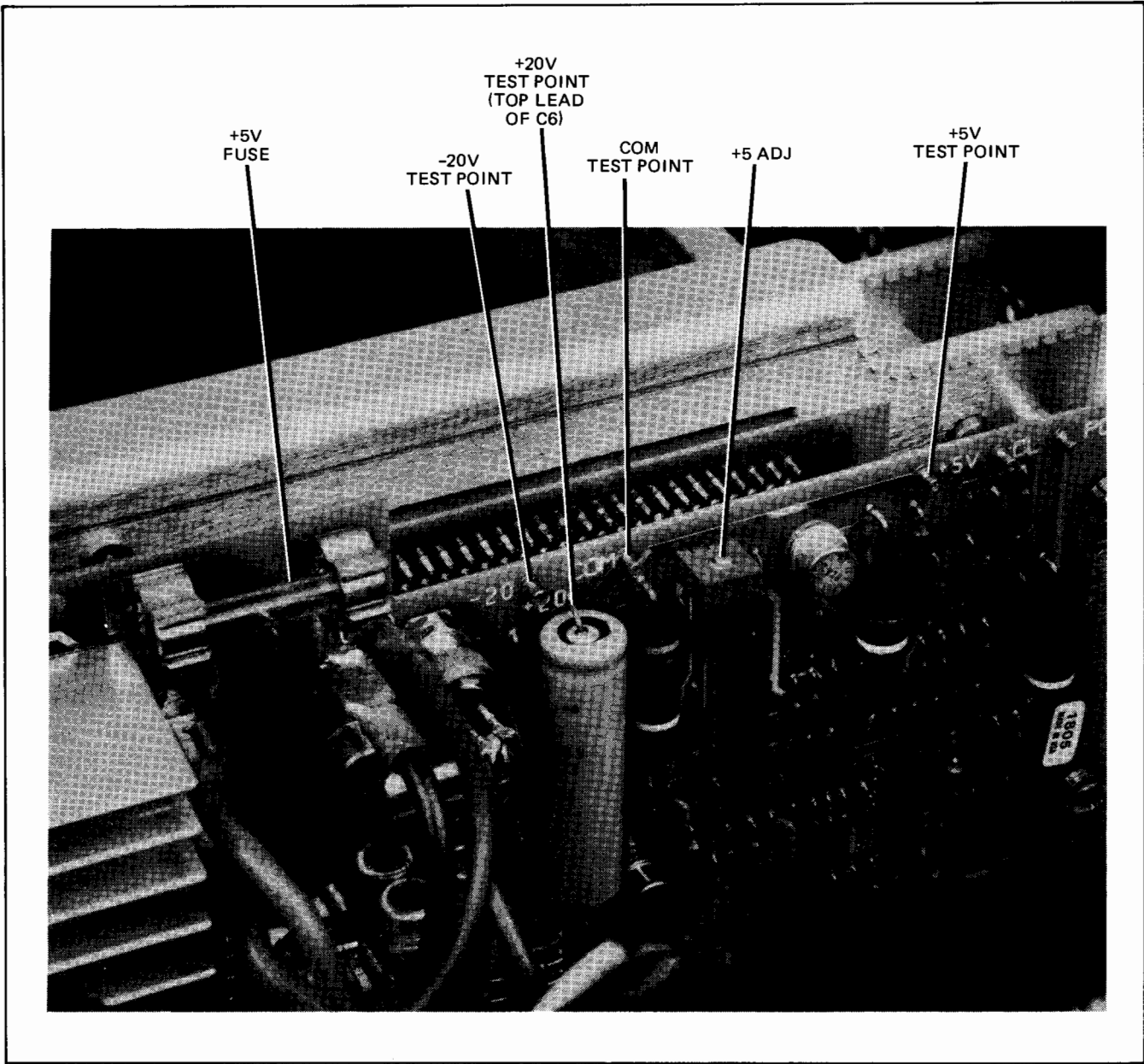
Figure 2-3. Power Supply Adjustment and Test Points
