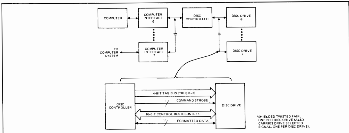
Figure 4-7. Controller/Disc Drive Interface Block Diagram
