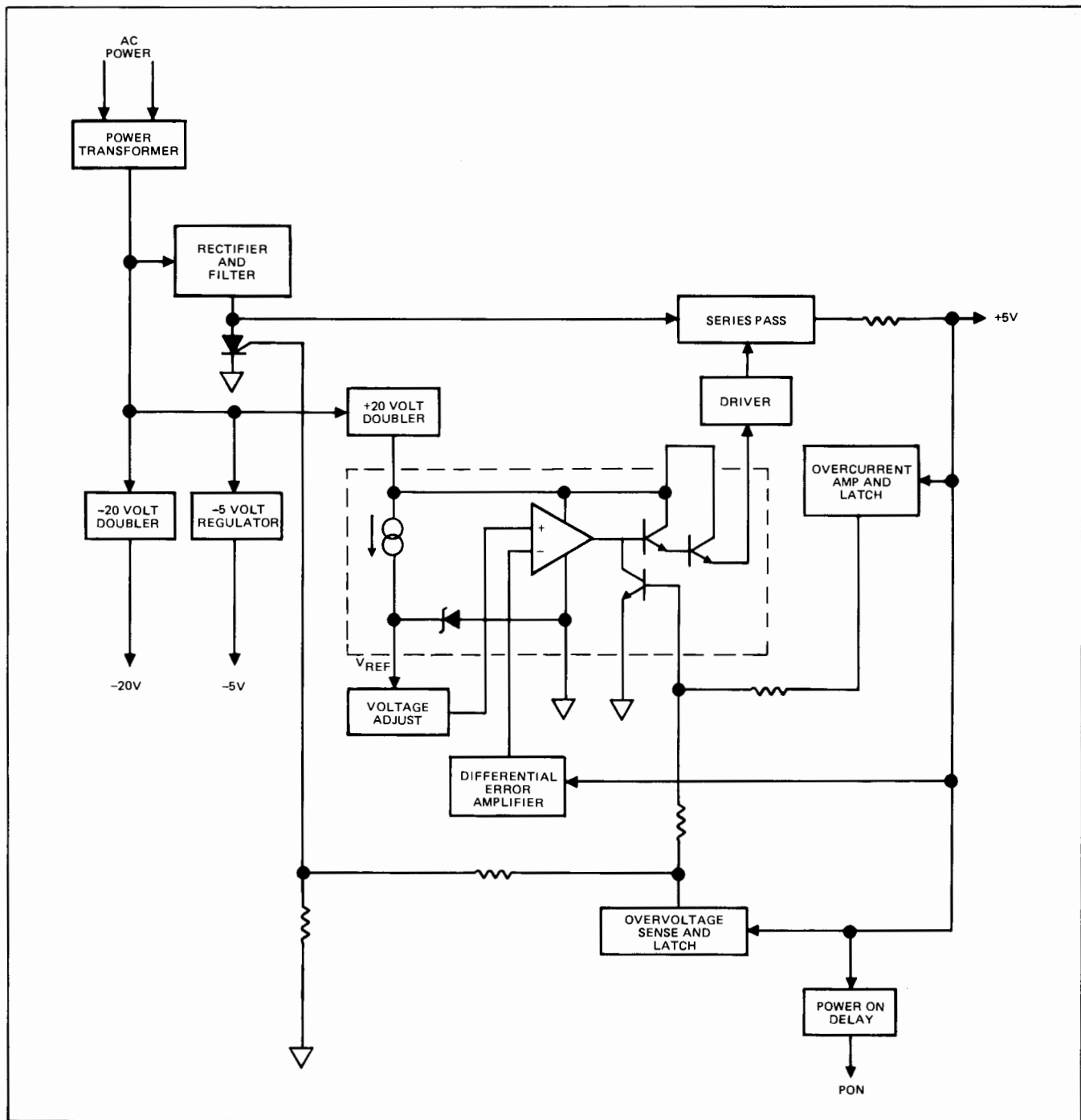
Figure 4-11. Power Supply Functional Block Diagram
