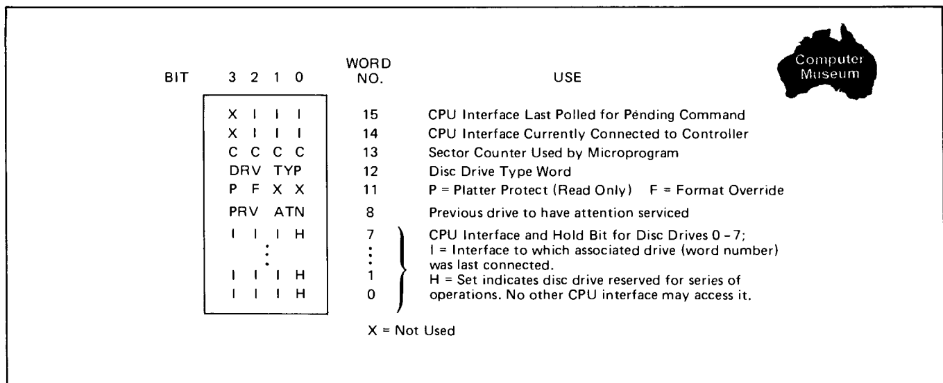
Figure 4-5. Diagram of Device Controller PCA RAM
