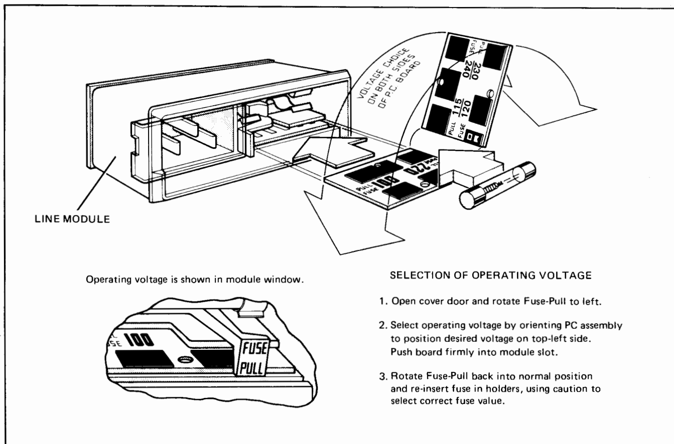
Figure A-1. Line Module Voltage Selection
