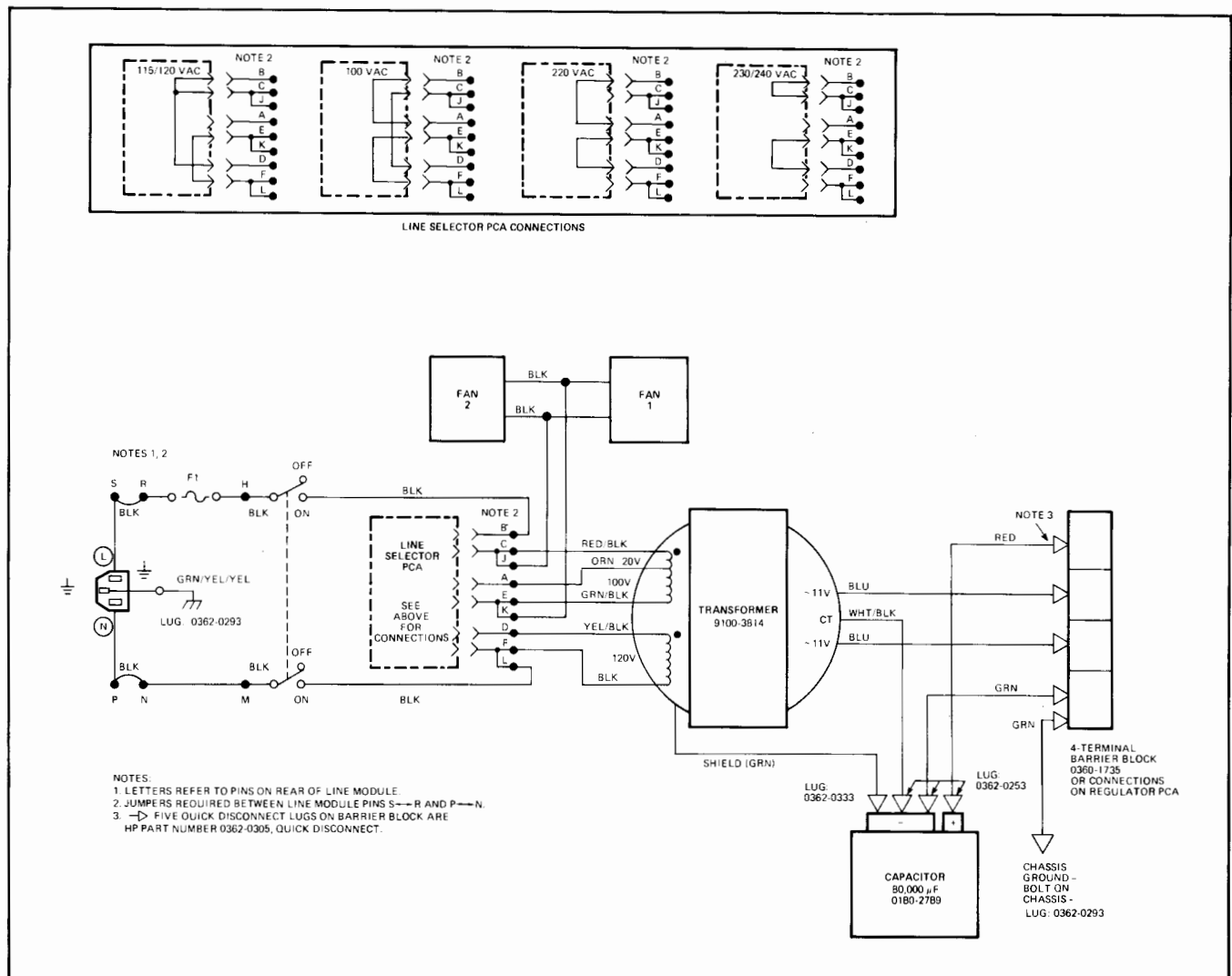
Figure A-5. Controller Power Distribution
