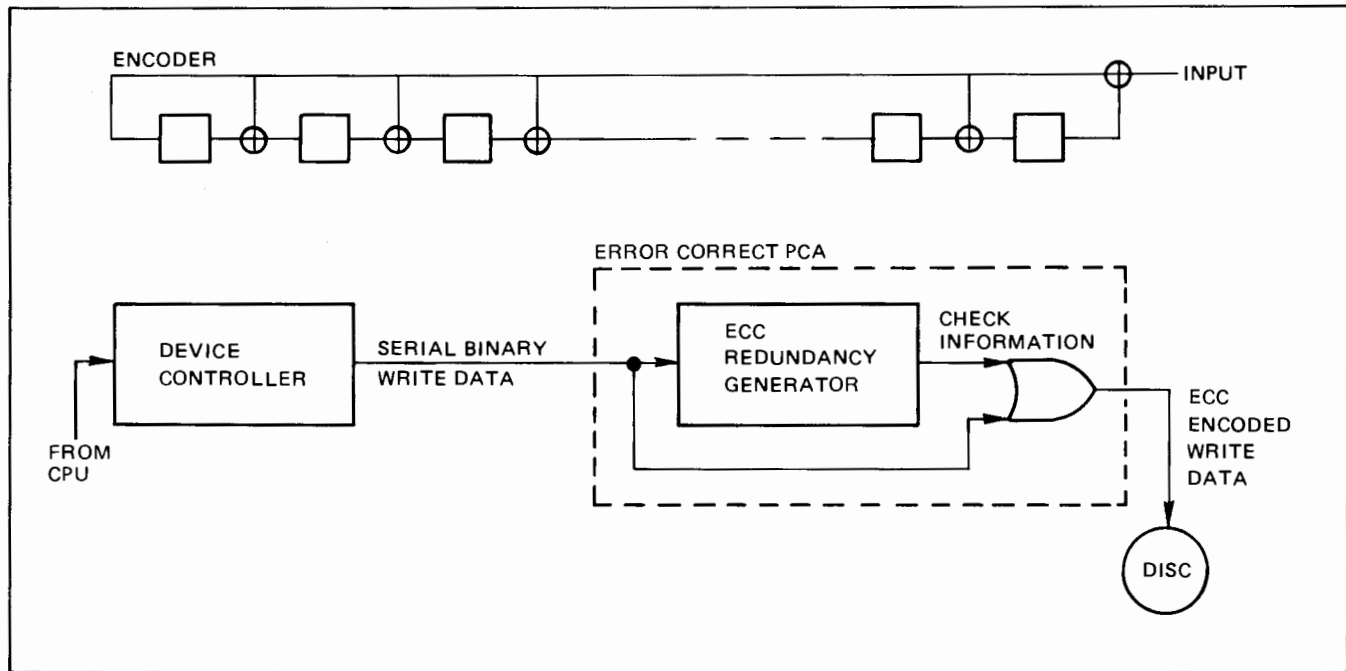
Figure 4-9. ECC Write Circuit
