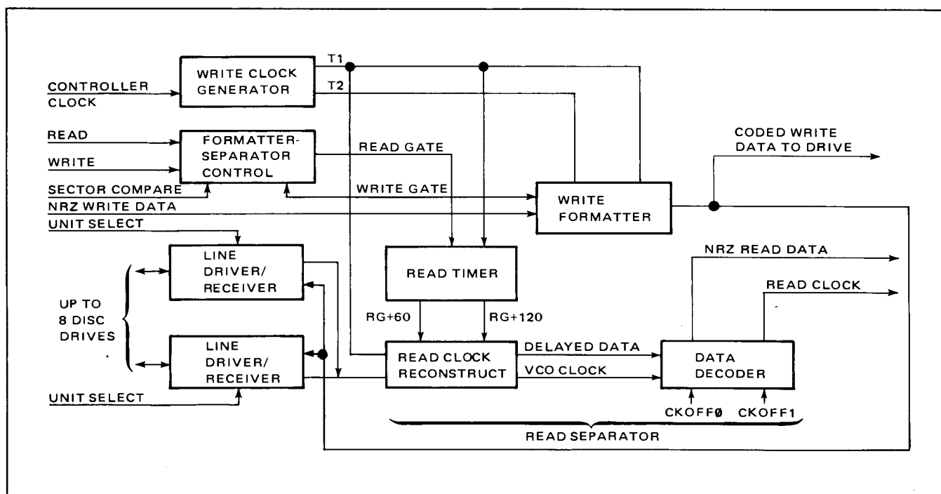
Figure 4-4. Data Formatter-Separator Block Diagram
