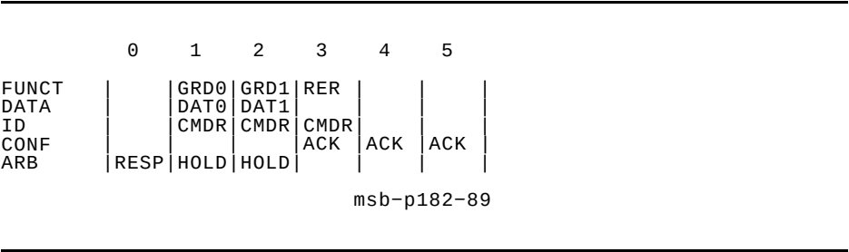
Figure 2–30 Hexword Data Return with Uncorrectable Read Error
