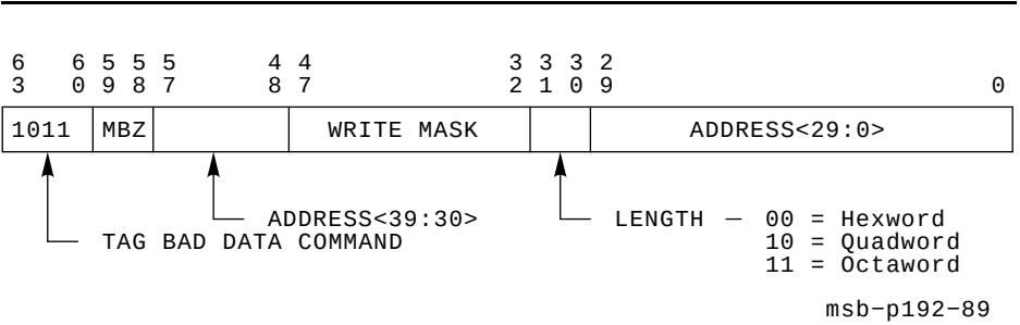
Figure 2–19 Tag Bad Data Command
