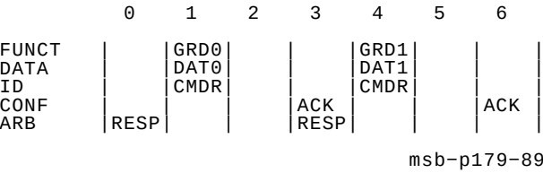
Figure 2–27 Four Longword Reads
