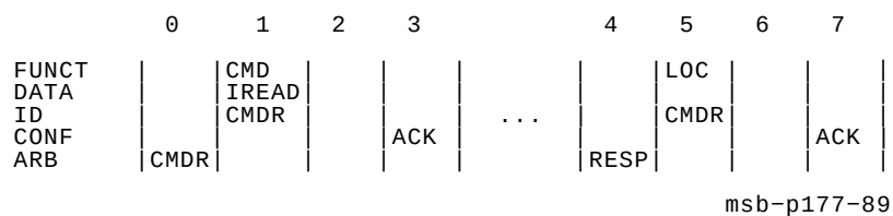
Figure 2–25 Interlock Read Transaction to a Locked Location
