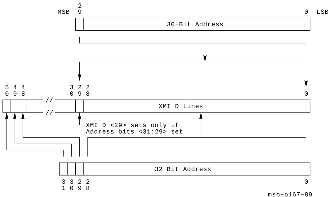
Figure 2-4 Address Association
