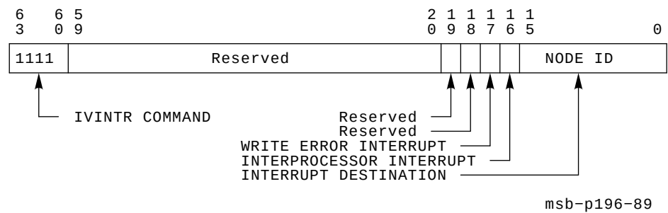
Figure 2–23 Implied Vector Interrupt Command
