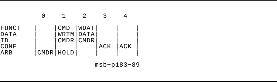
Figure 2–31 Longword and Quadword Writes
