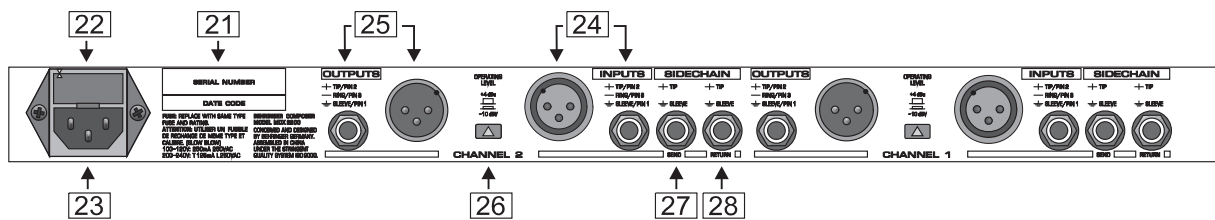
Fig. 2.5: Control elements of the rear panel
