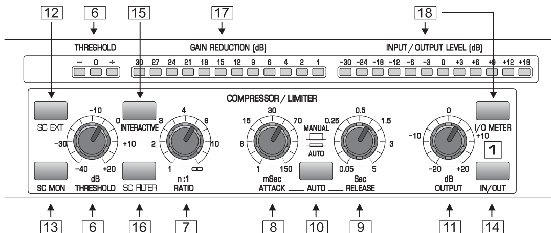
Fig. 2.3: Control elements of the compressor section
