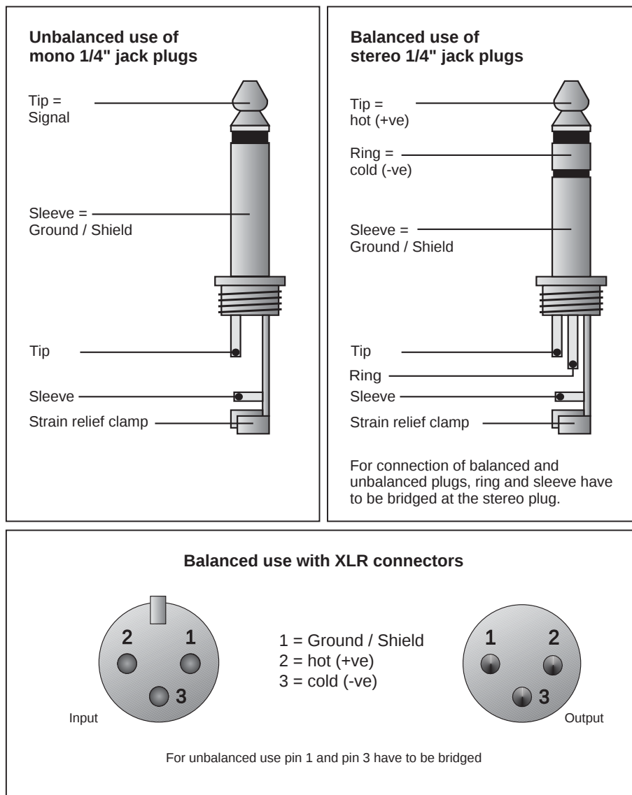
Fig. 7.2: Different plug types
