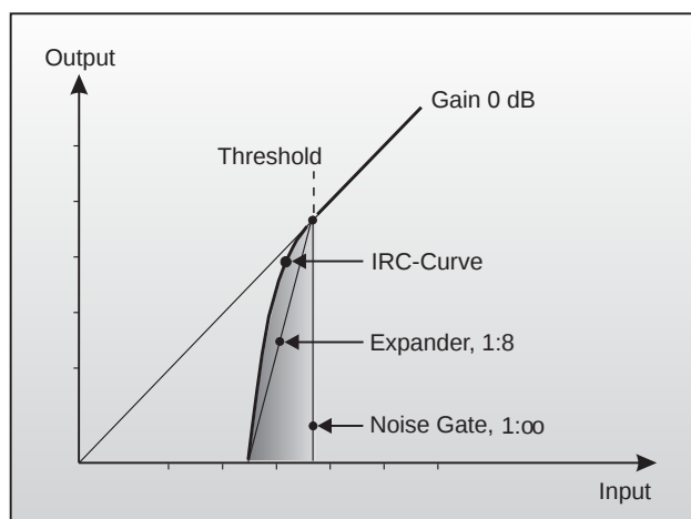
Fig. 4.1: IRC curve characteristic of the Expander
