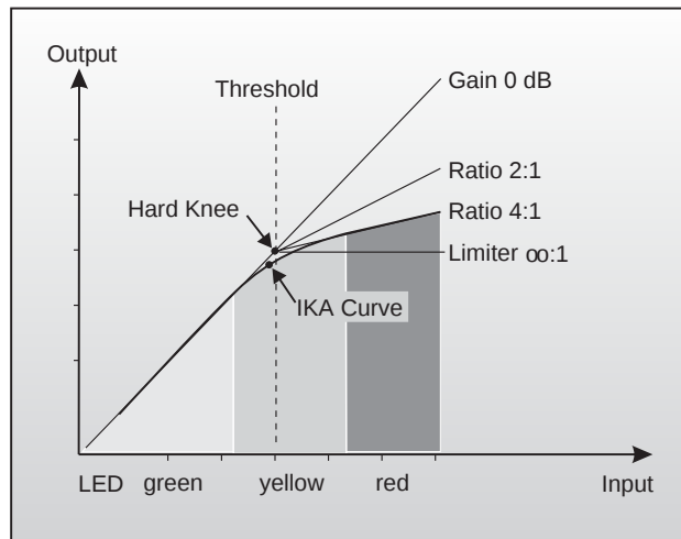
Fig. 4.2: IKA characteristic of the compressor section
