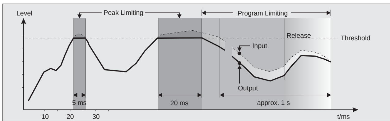
Fig. 4.3: IGC characteristic of the limiter section
